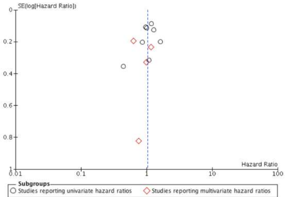
Supplementary Fig 6. Funnel plot based on meta-analysis comparing survival of patients aged above the median age reported in each study to those aged below the median age
